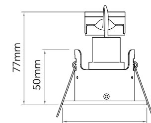
Bezel Diameter 81.5mm Cut Out Ø 55-68mm
